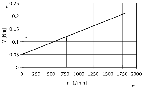
No-load torque: EXCM-30
