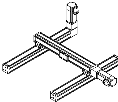
Complete system comprising motor, motor controller and motor mounting kit Motor
